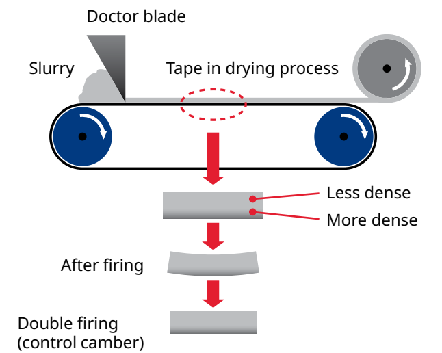
Classic method: Doctor blade method (DB)
